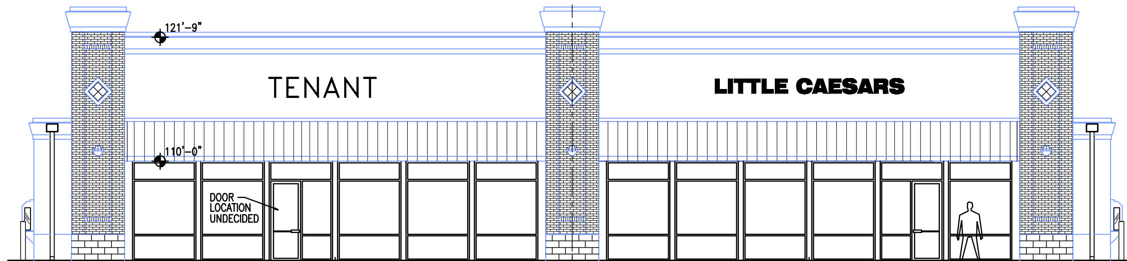
SOUTH ELEV 1/8"
